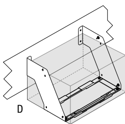
CHASSIS support bracket kits for Mother Trucker , Origin and Day Trippin'
