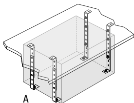
PLATFORM support bracket kits for Black Dog and Vertigo
